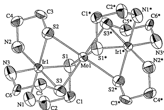
Fig. 2 Perspective view of \Delta\Delta\text{-}[\text{Mo}\{\text{Ir}(\text{aet})_3\}_2]^{4+} 1 with the atomic labeling scheme.
