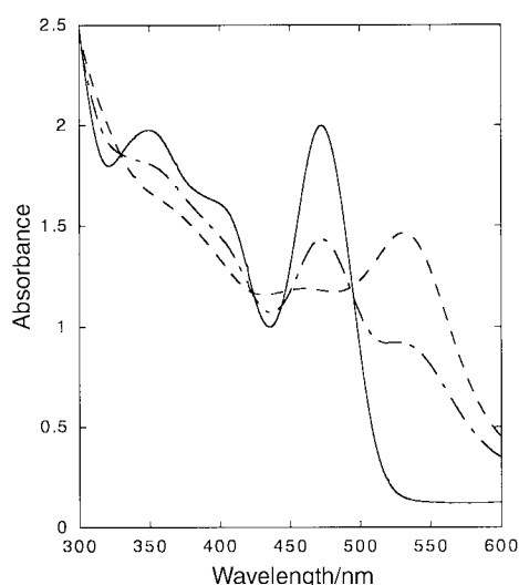
Fig. 1 Absorption spectral changes with times of [\text{Mo}\{\text{Rh}(\text{aet})_3\}_2]^{3+} 2; 0 (—), 4 (---), and 16 h (— · —).
