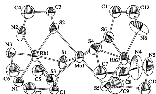
Fig. 3 Perspective view of \Delta\Delta\text{-}[\text{Mo}\{\text{Rh}(\text{aet})_3\}_2]^{3+} 2 with the atomic labeling scheme. The overlapped \Delta\Delta isomer is omitted for clarity.
