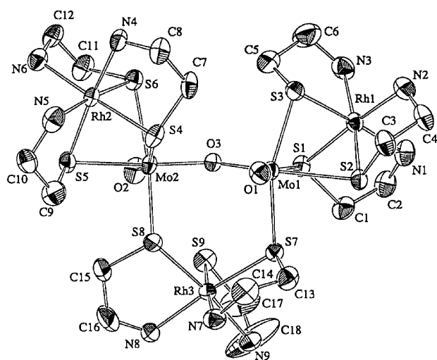
Fig. 4 Perspective view of ΔΔΔ-[Mo 2 O 2 (μ-O){Rh(aet) 3 }] 4+ 3 with the atomic labeling scheme.
